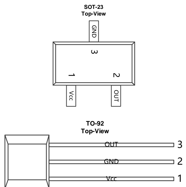
Figure.1 Pin Configuration & Functions
